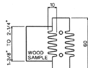
50 mm Joint #602005, #602213
