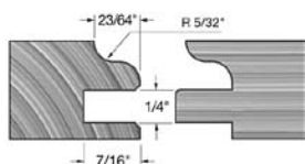
RAISED PANEL PROFILES For thickness 3/4" to 7/8"
