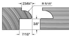
GLASS PANEL PROFILES For thickness 3/4" to 13/16"
