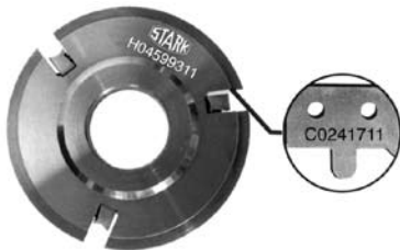
GROOVE CUTTERHEAD BODY (Insert knives sold separately)
