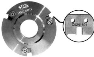
TONGUE CUTTERHEAD BODY (Insert knives sold separately)
