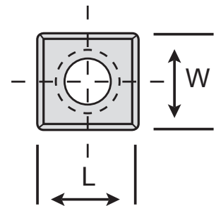
IN151525(R) Radiused Corners
