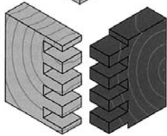
5/16" or 1/2" Box Joint
