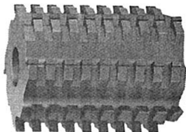
Carbide Tipped Staggered Tooth Moulder Head CT/STMH 6" Diameter x 1-13/16" Bore
