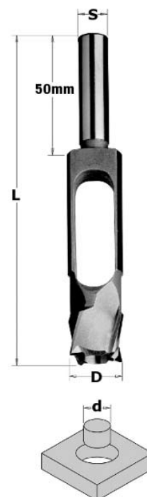
Plug Cutter
